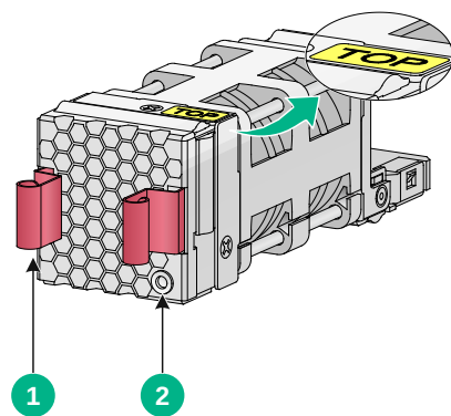
图1-8 FAN-40B-1-A-Z 风扇模块
